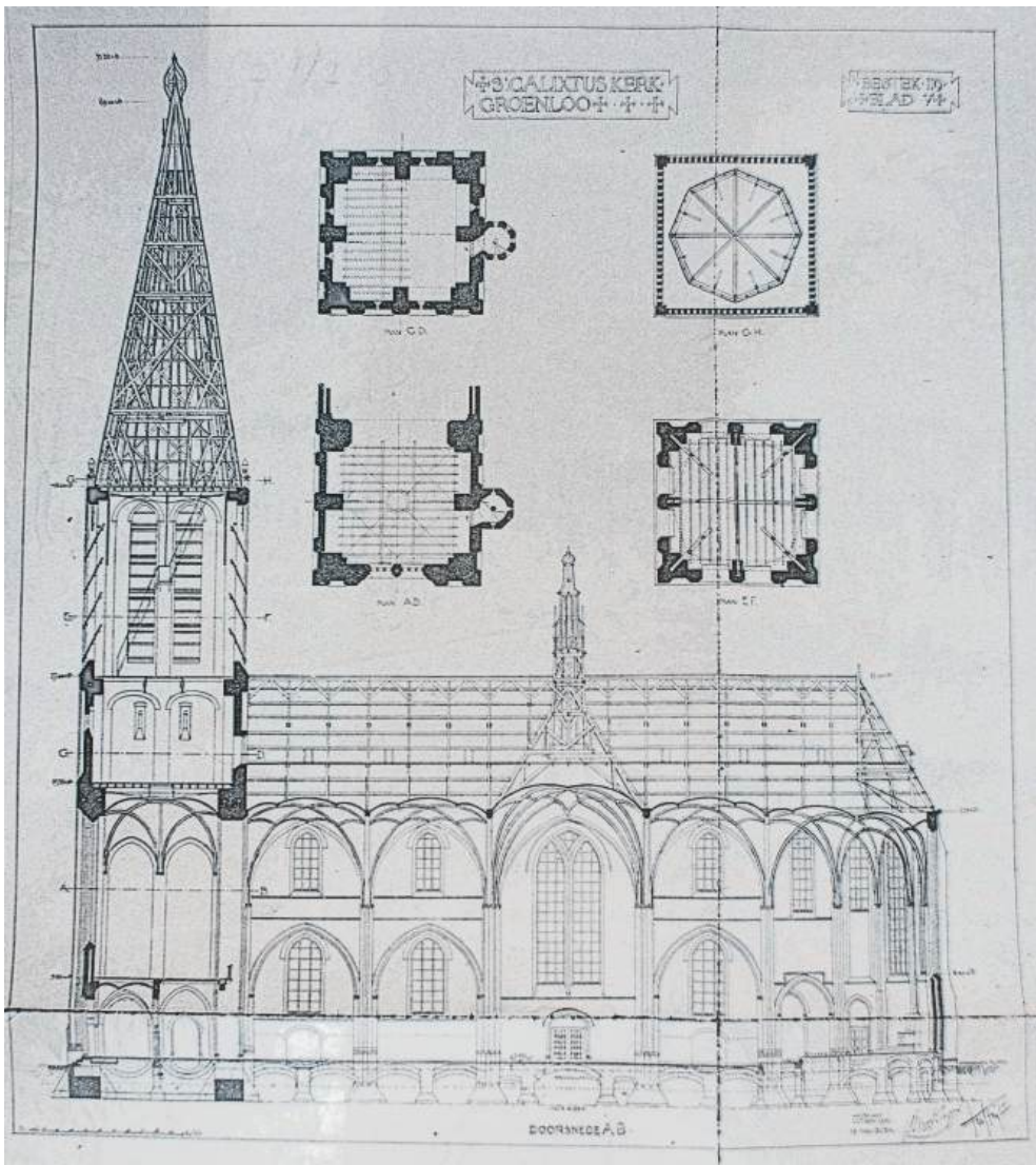
Doorsnede (bron ECAL)
